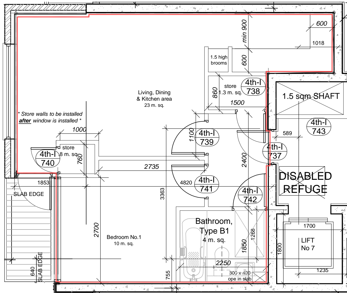
Fourth Floor Residential Layout Apartment No. 511 (1 Bed) Area: 45 m 2
